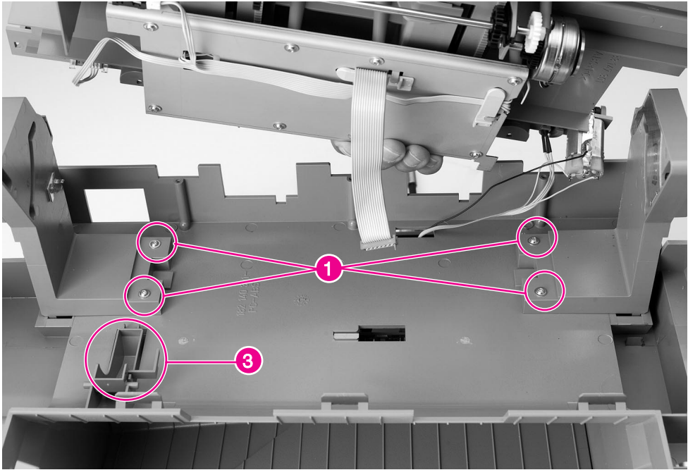
Figure 6-189 Hinges
