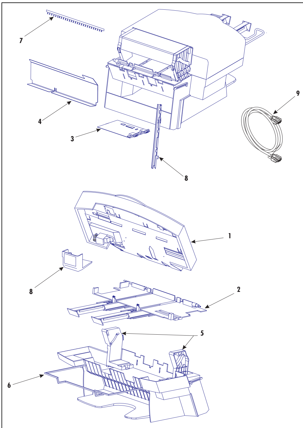
Figure 8-15 Stapler Internal Components
