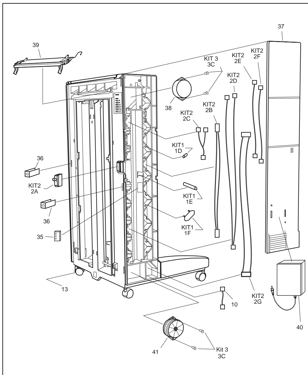
Figure 8-14 8-bin Mailbox Components (3 of 3)
