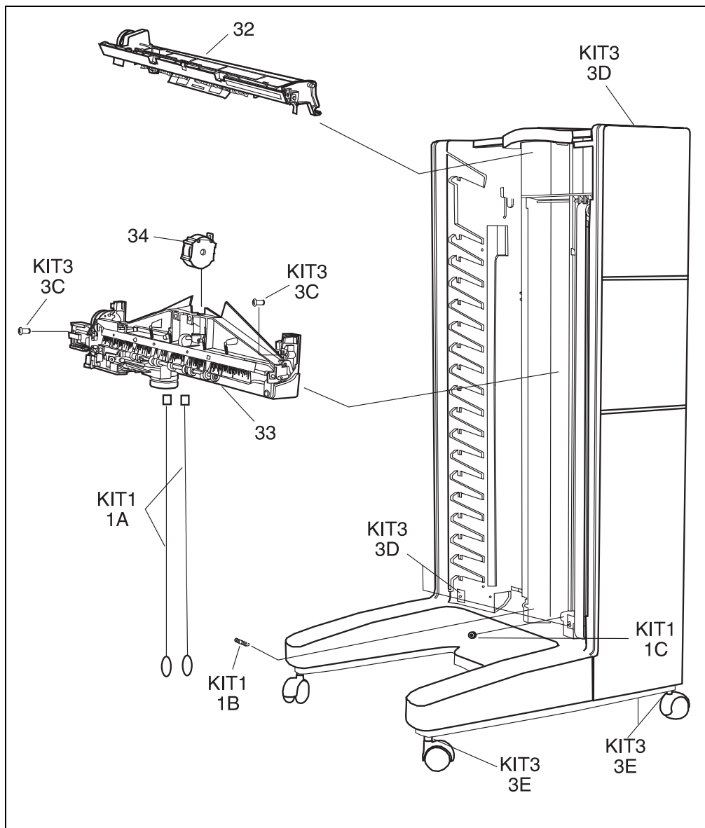
Figure 8-13 8-bin Mailbox Components (2 of 3)
