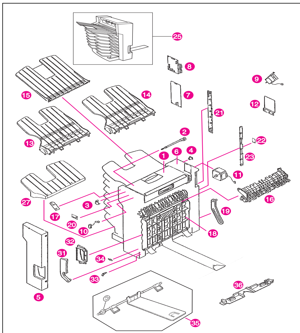
Figure 8-17 7-bin Tabletop Mailbox Internal Components
